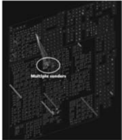
Figure 2. Itoh, et al. 2006, visualization display. The color of the extruded bars correspond to the number of sent and received incidents.
