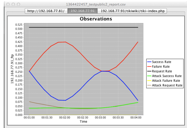
Figure 3. Baseline performance of the vulnerable FTP service subject to fixed rates of legitimate and malicious traffic.
