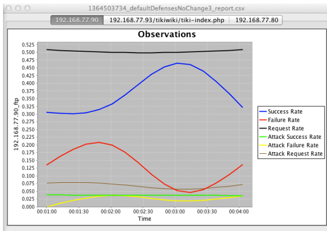
Figure 5. Effects of the Application Diversity Defense configured by the MTC2 for a balanced 30-second interval.
