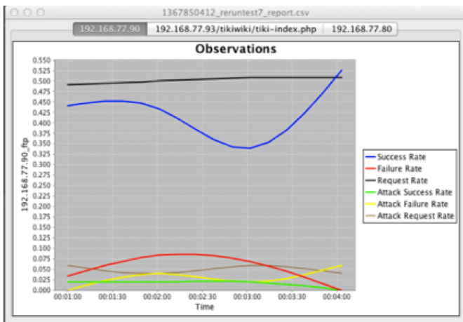
Figure 9. Example output showing the results of modifying the time between application changes
