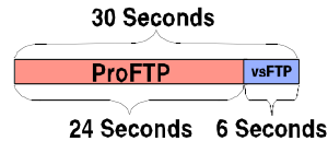
Figure 6. Biased switching schedule for Application Diversity defense of FTP service.
