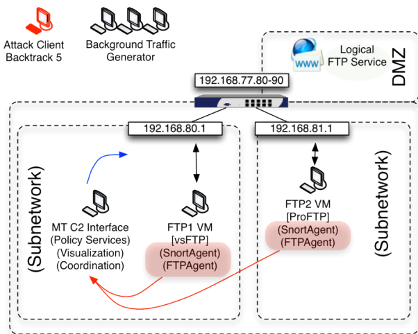
Figure 2. Partial Network topology showing the FTP services involved in the example MTC2 scenario.
