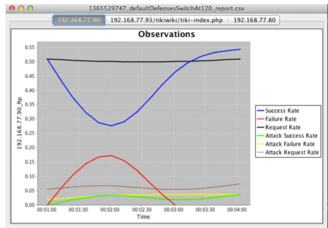
Figure 7. Effects of the Application Diversity Defense configured by the MTC2 for a 80%-20% split, with a 30 second interval
