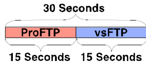
Figure 4. Balanced switching schedule for Application Diversity defense of FTP service.
