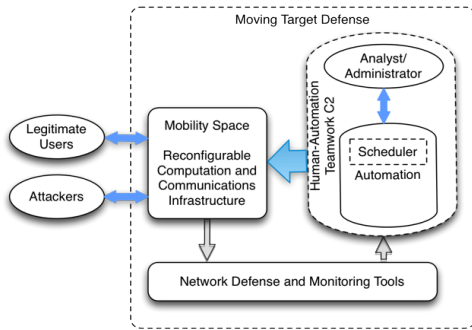
Figure 1. A Human-Agent Teamwork Approach to MTC2
