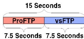
Figure 8. Higher frequency, balanced switching schedule for Application Diversity defense of FTP service.
